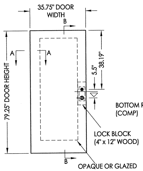
STEEL DOOR PANEL Masonite 6' 8" (Wood Edge)
