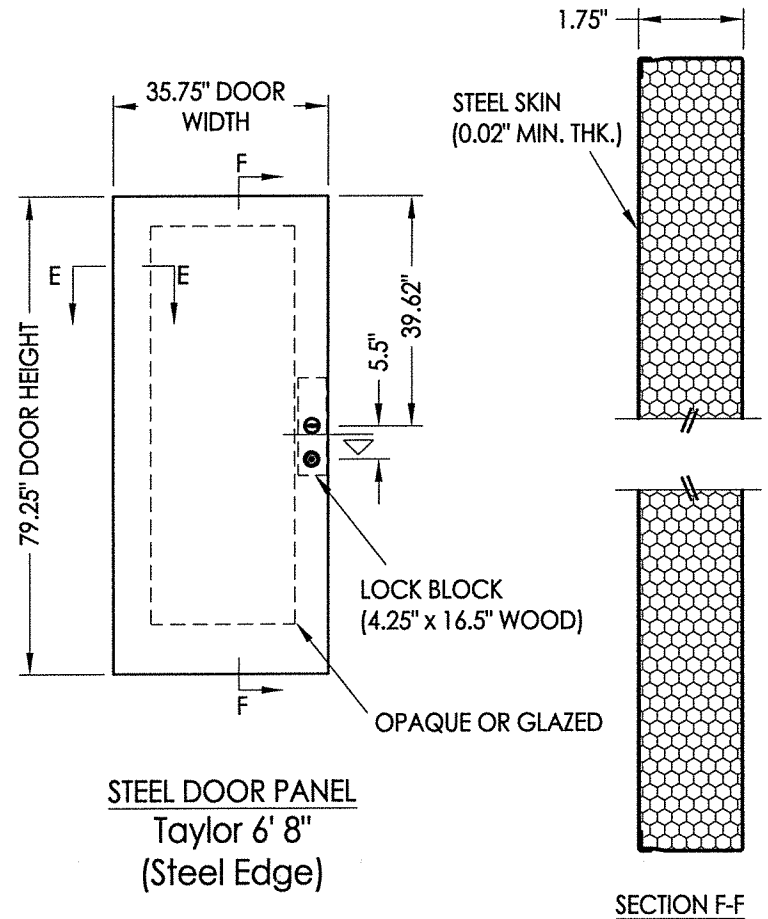
SECTION F-F
