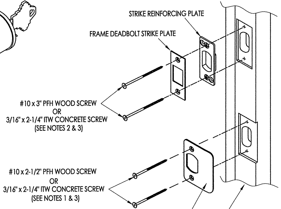
SINGLE DOOR WOOD FRAME INSTALLATION DETAILS
